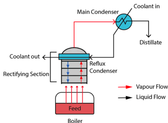
Figure 2. Schematic representation of the batch distillation apparatus, illustrating vapor flow from the boiler through the rectifying section and condensation in the reflux and main condensers, with the indication of resulting distillate and reflux streams
