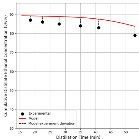
Figure 8. Cumulative distillate ethanol concentration versus distillation time for Run 3. Experimental cumulative concentrations are compared with the model prediction; dashed vertical lines indicate the model-experiment deviation.
