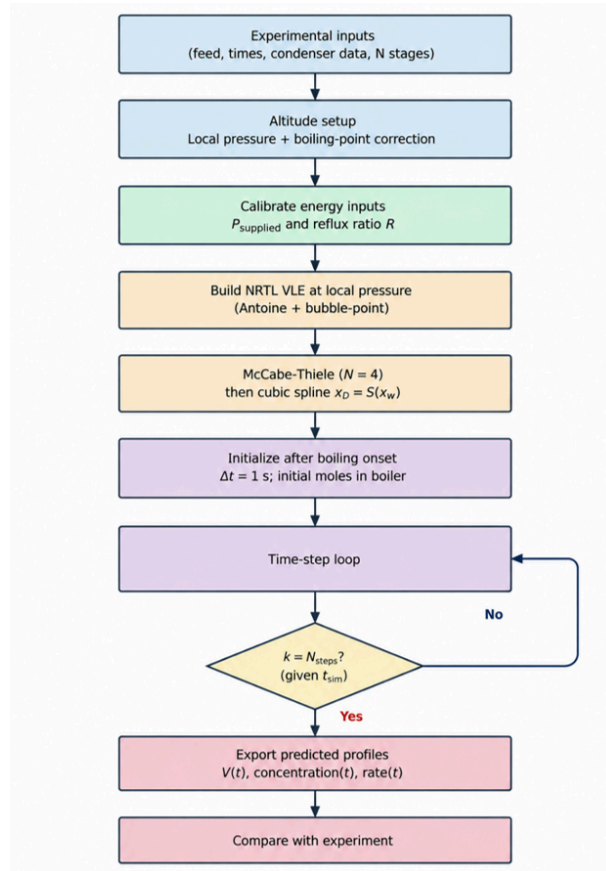
Figure 1. Flowchart of the NRTL batch-distillation solver: altitude-corrected VLE and energy calibration, McCabe-Thiele spline construction, and the 1-second time-stepping loop used to predict distillate volume and composition
