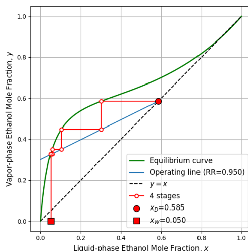
Figure 5. McCabe - Thiele diagram for Run 3 illustrating the equilibrium curve, operating line, and four theoretical stages (reflux ratio = 0.950)
