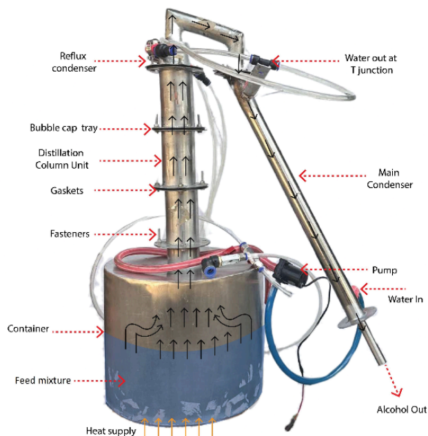
Figure 4. Fabricated prototype of the developed batch distillation apparatus for ethanol - water separation.
