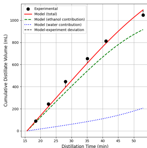
Figure 7. Cumulative distillate volume versus distillation time for Run 3. Experimental cumulative distillate volumes are compared with model predictions; dashed vertical lines indicate the model-experiment deviation.
