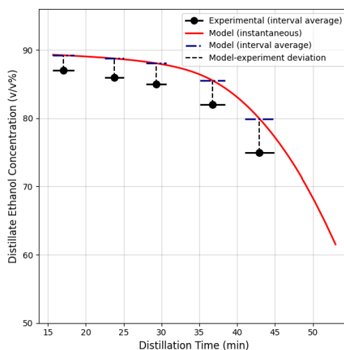
Figure 9. Comparison of experimental and model-predicted distillate ethanol concentration with distillation time for Run 3. Experimental interval-average values, instantaneous model predictions, interval-average model predictions, and model–experiment deviations are shown.
