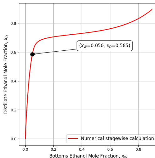
Figure 6. Relationship between bottoms ethanol mole fraction and distillate ethanol mole fraction for Run 3, obtained from the four-stage McCabe–Thiele stage-stepping calculation at a reflux ratio of 0.950.
