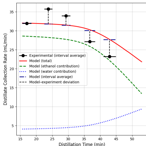
Figure 10. Distillate collection rate versus distillation time for Run 3. Experimental interval-average rates are compared with model-predicted total, ethanol, water, and interval-average rates; dashed vertical lines indicate the model–experiment deviation.
